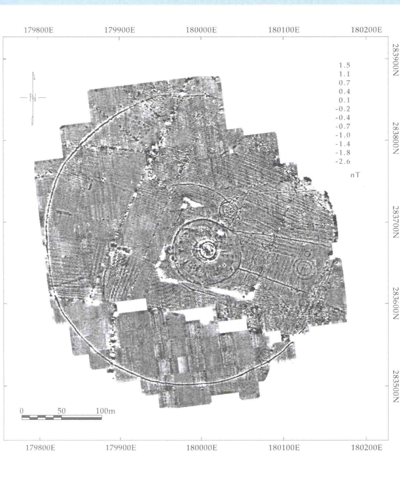
Geophysical survey: Rathcroghan Mound and the 360m enclosure.
