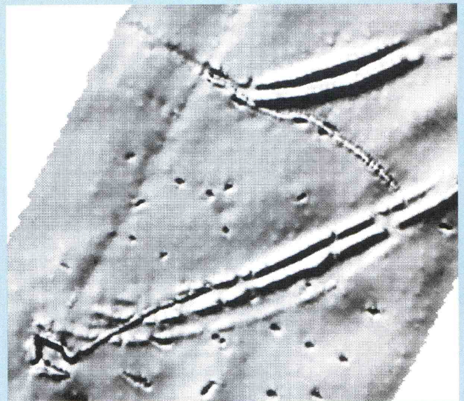
The Mucklaghs: geophysical image showing linear earthworks.
